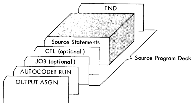
Figure 11. AUTOCODER RUN
