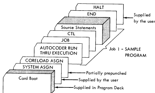
Figure 31. Sample Program
